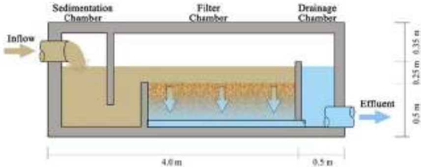
Figure 13.1 The innovative sand filter system (figure by authors).
